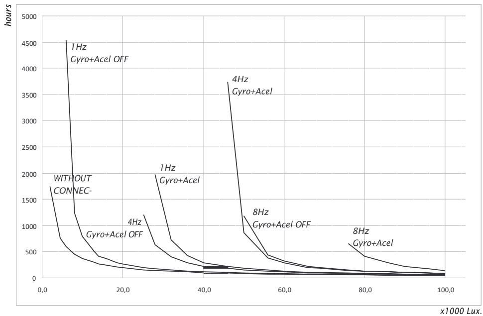
Graphic 2. Load hours/Illuminance -DEPPENDING ON THE USE OF ULTRASONIC DEVICE
